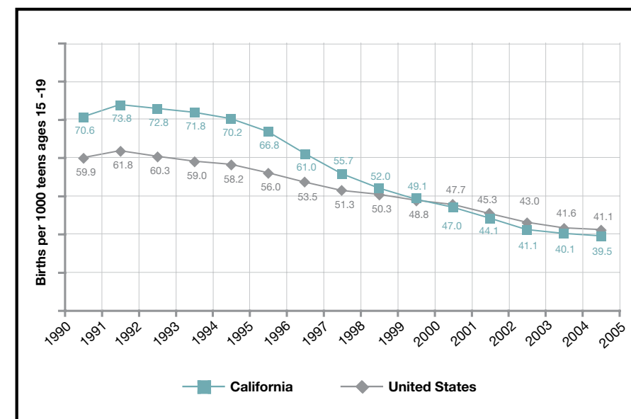
Trend in Teen Birth Rates: California vs. US
